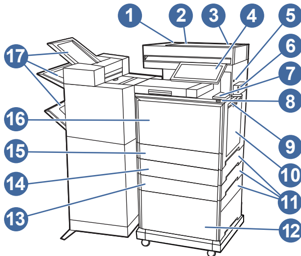
Figure 1-7 Printer front view - z+ models
