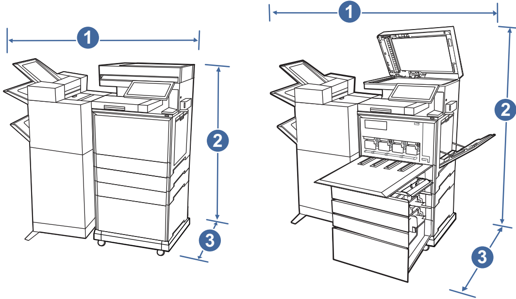
Figure 1-12 Printer dimensions (z+ models)
