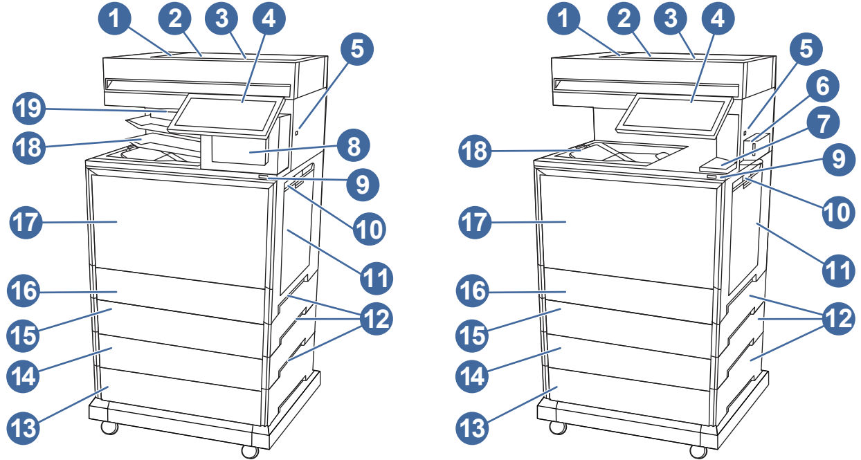
Figure 1-6 Printer front view - dn and zs models
