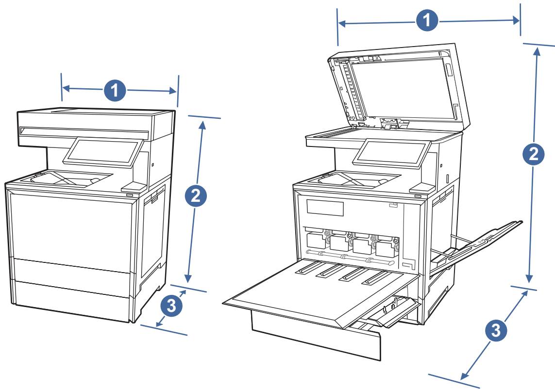
Figure 1-10 Printer dimensions (dn, s, and z models)
