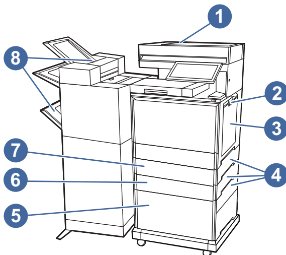
Figure 8-11 Paper jam locations - z+ models
